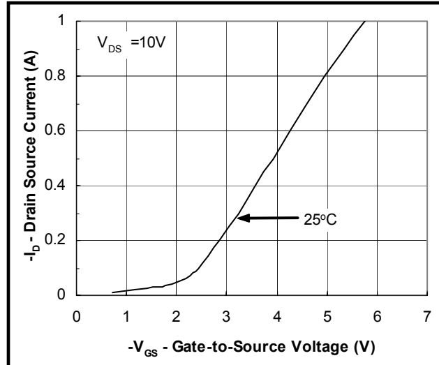
Fig. 2. Transfer Characteristics
